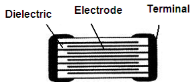
Inner Structure
